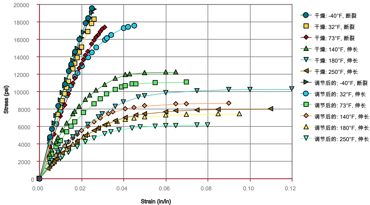
等温应力与应变 (ISO 11403-1)
